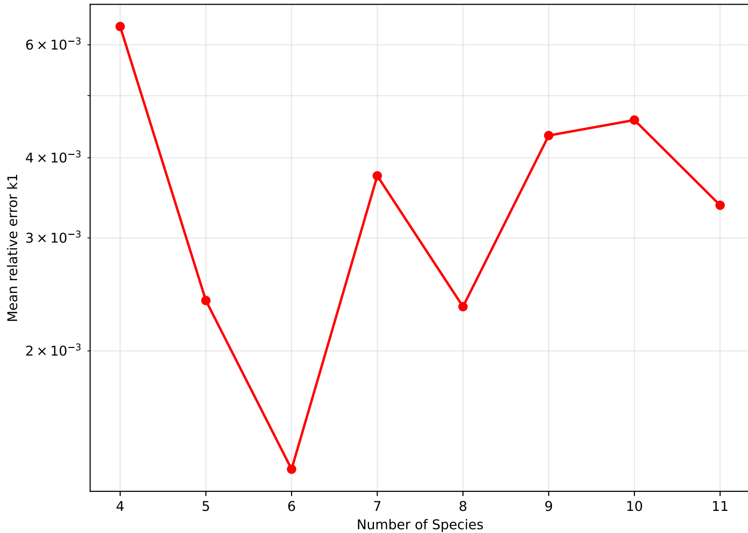
50, 50 — Mean relative error k1 vs number of species (zoomed: 4 to 11 species)
